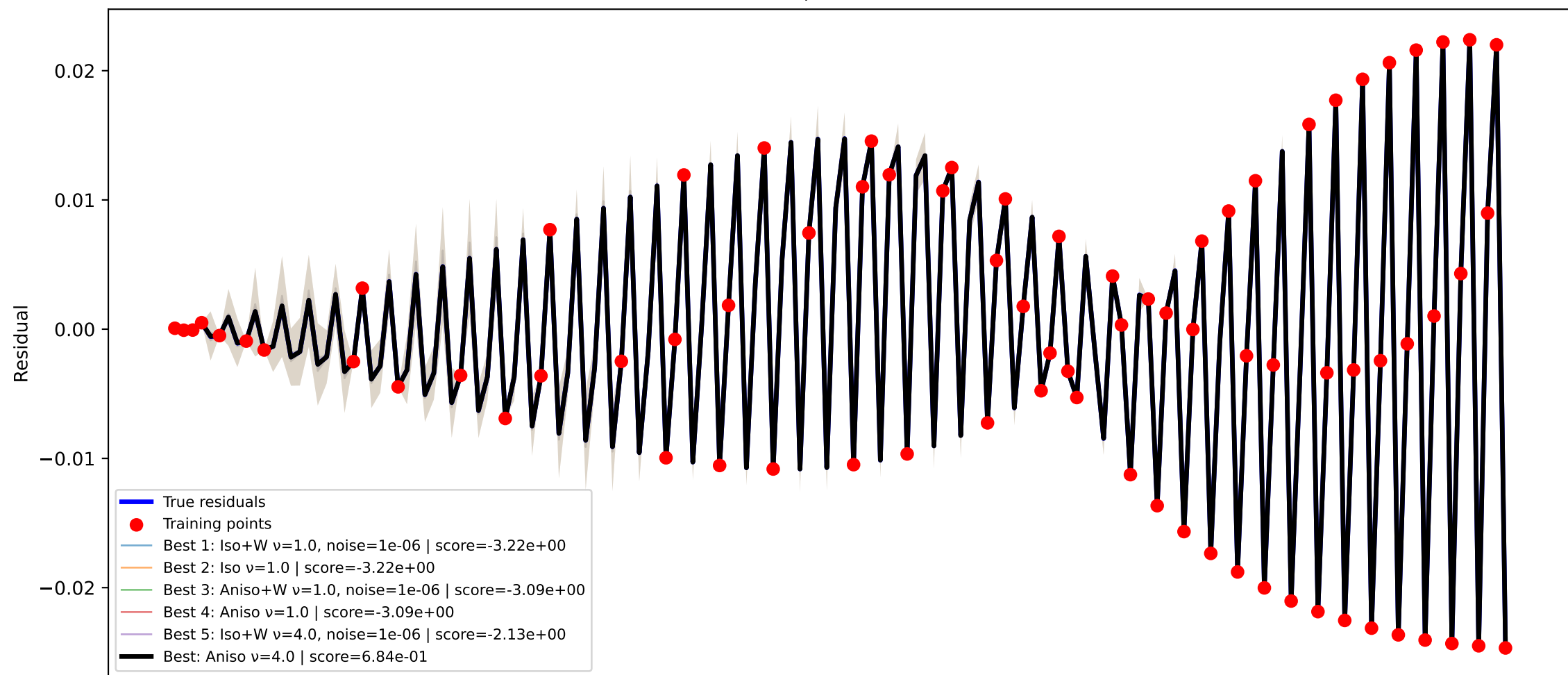
GPR kernel comparison node=31 RMSE=8.052e-06, train RMSE=2.566e-09
